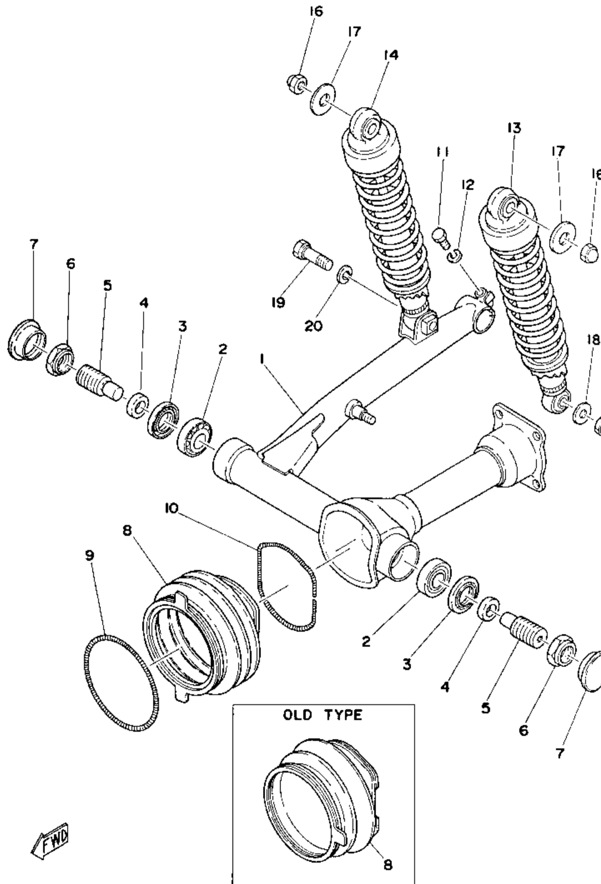
Fig. 26 REAR ARM - REAR CUSHION
