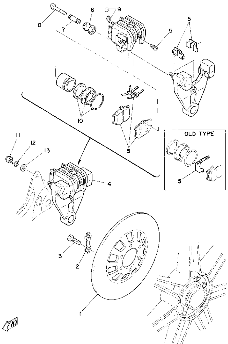
Fig. 39 REAR DISK BRAKE - CALIPER
