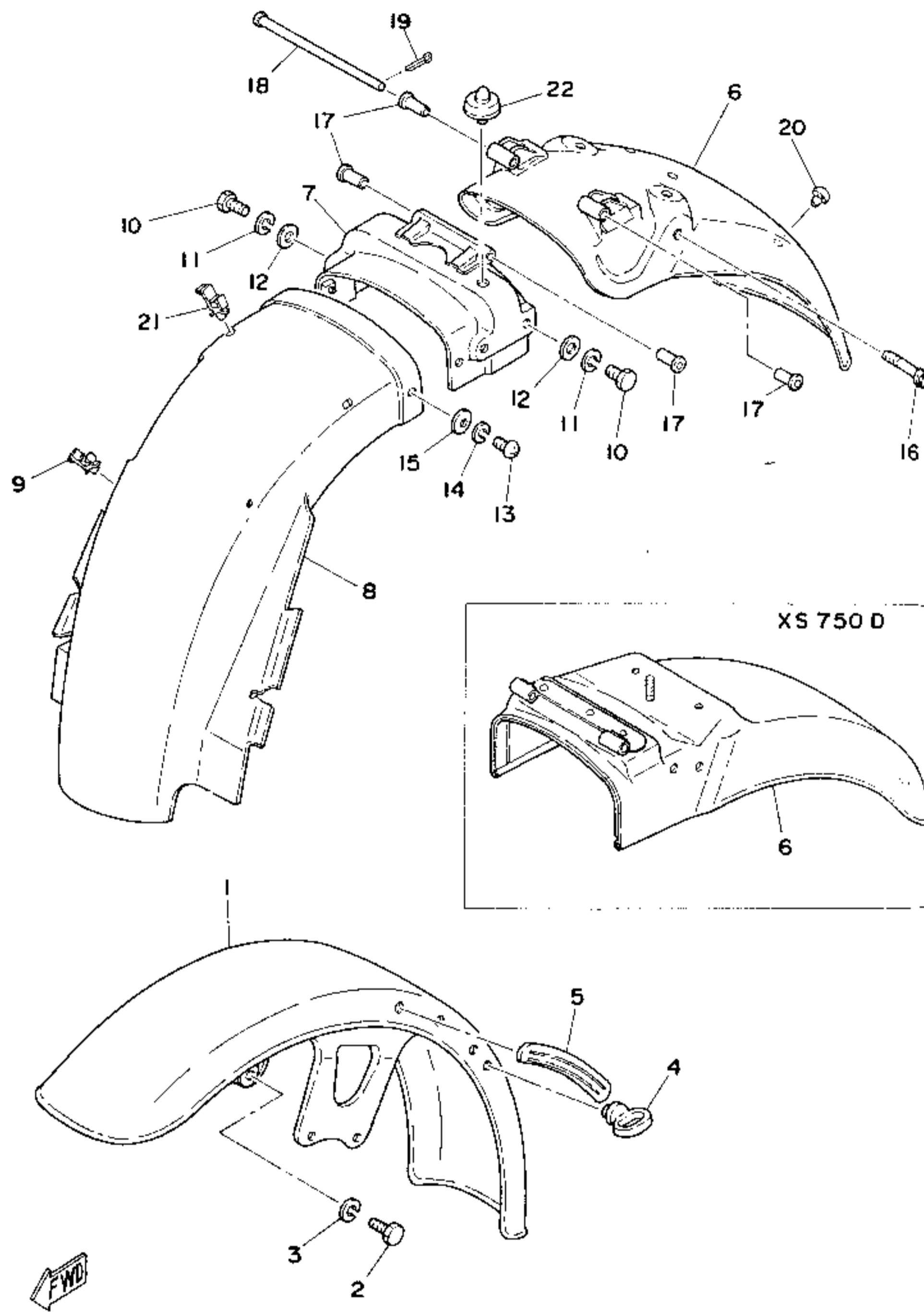
Fig. 27 FRONT FENDER · REAR FENDER
